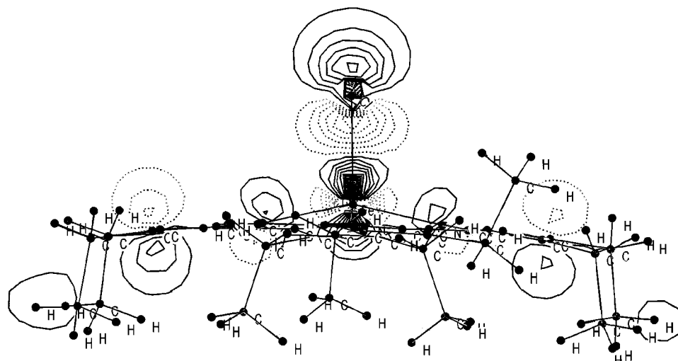
Figure 9. Calculated electron-density contour map of HOMO-3 ( 162\alpha with Fe d_{z^2} , Cl p_z contributions) for [FeCl(OECorr)].
