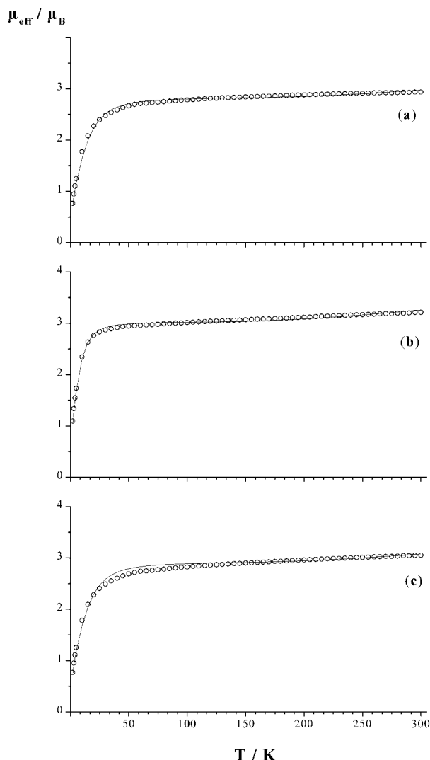
Figure 2. Temperature dependence of the effective magnetic moment \mu_{\text{eff}} of (a, c) [FeCl(7,13-Me 2 Et 6 Corr)] and (b) [FePh(7,13-Me 2 Et 6 Corr)] obtained in a field of B = 5 T and corrected for diamagnetic contributions only, i.e. TIP = 0. The solid lines are fits (based on the spin-Hamiltonian approach) assuming antiferromagnetically exchange-coupled Fe(III) S_1 = 3/2 corrolate \pi -cation radical ( S_2 = 1/2 ) species. The obtained parameters are the following: (a) J = 350 \text{ cm}^{-1} , D = 28 \text{ cm}^{-1} , g = 2.00 for [FeCl(7,13-Me 2 Et 6 Corr)], (b) J = 300 \text{ cm}^{-1} , D = 15 \text{ cm}^{-1} , g = 2.11 for [FePh(7,13-Me 2 Et 6 Corr)], and (c) J = 343 \text{ cm}^{-1} , D = 28 \text{ cm}^{-1} (fixed), g = 2.05 (fixed) for [FeCl(7,13-Me 2 Et 6 Corr)].
