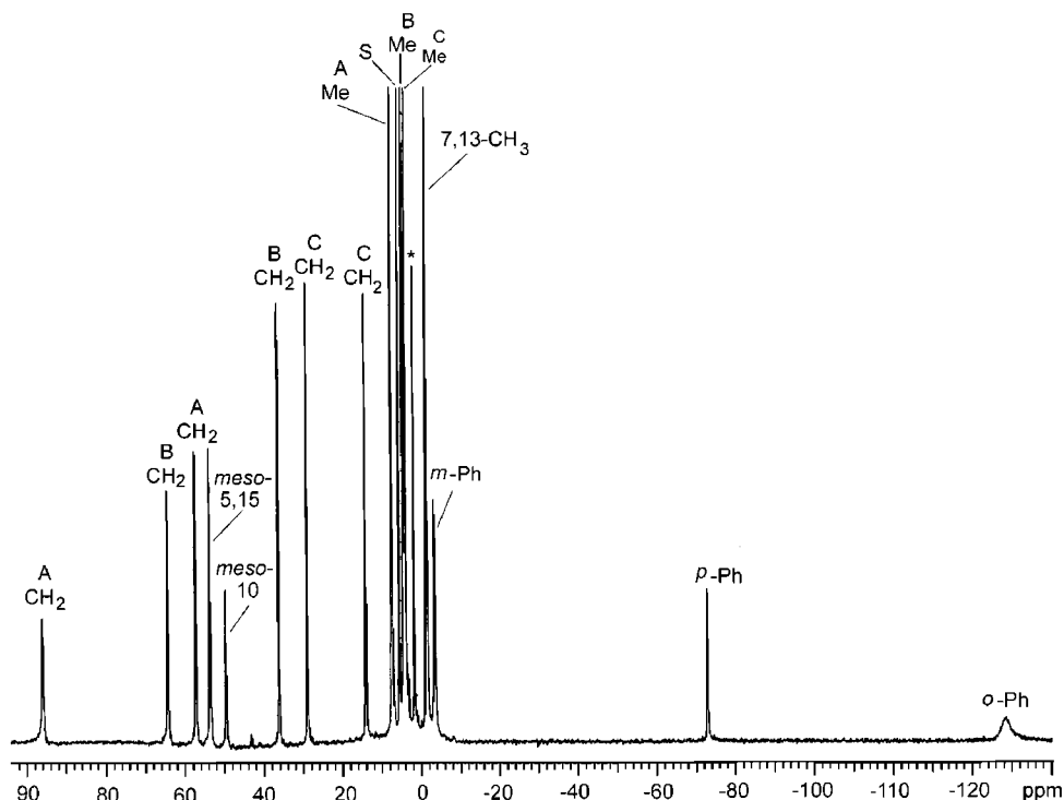
Figure 5. 1D ^1\text{H} NMR spectrum of [\text{FePh}(7,13\text{-Me}_2\text{Et}_6\text{Corr})] in \text{CD}_2\text{Cl}_2 at 30\text{ }^\circ\text{C} . J -coupled ethyl groups are shown by the letters A, B, and C.
